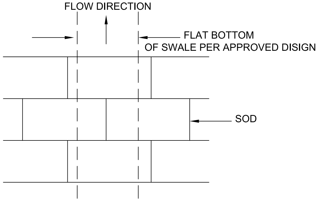
VEGETATED SWALE PLAN VIEW
