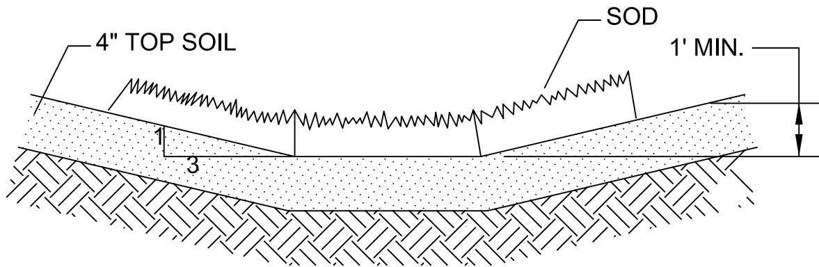
VEGETATED SWALE CROSS SECTION
