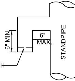
ELBOW DETAIL
