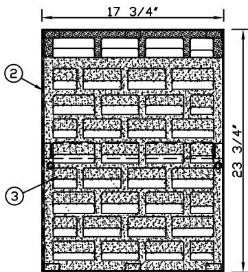
SECTION A-A GRATE RAISED
