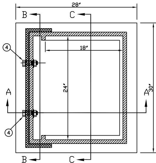
TOP VIEW GRATE REMOVED
