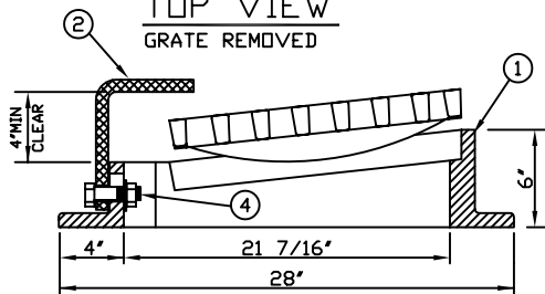
SECTION A-A GRATE RAISED
