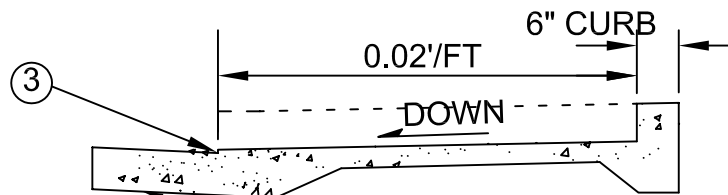
TYPE A CURB & GUTTER STD DETAIL 3-6
