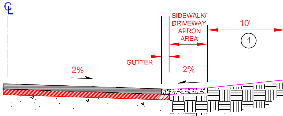
PLAN
